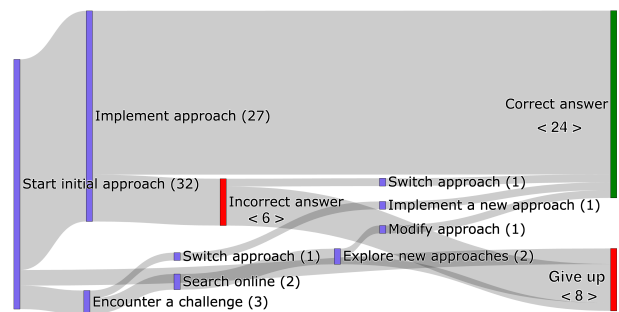
Figure 2: This Sankey diagram shows the progress of participants for the Format task. Each node represents the activity and the number of participants. The edges represent the orders of activities.
