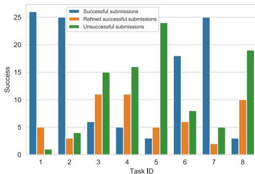
Figure 3: The distribution of cases for 1). Successful submissions, 2). Refined successful submissions, and 3). Unsuccessful submissions categories across eight tasks.
