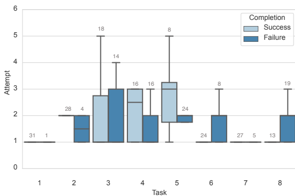
Figure 1: A boxplot showing how the number of attempts differs across success and failure groups for the eight tasks. The numbers on top of whisker lines refers to number of participants that succeeded or failed.
